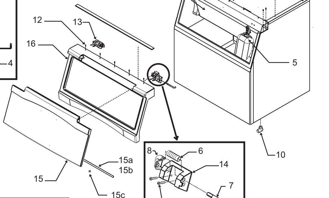
Hinge Detail
