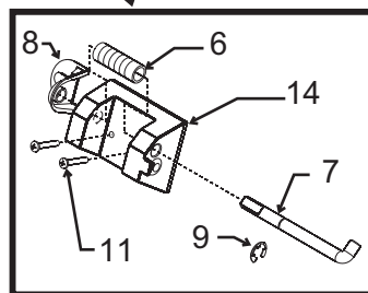
Hinge Detail
