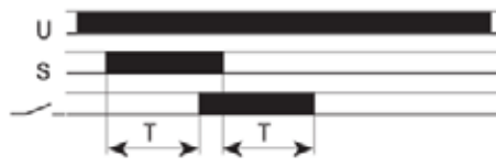
FZ16: ON Delay (1 timed contact + 1 instantaneous contact)
