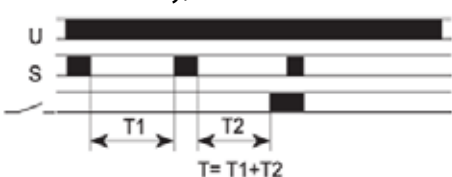
FZ09: ON delay, additive
