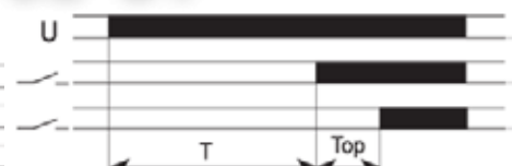
FZ27: 1 relay ON delay, 1 relay OFF delay
