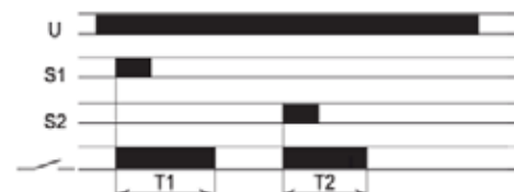
FZ32: Clock generator - Start after impulse
