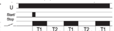
FZ39: Symmetrical recycling, ON start with Start/Stop pushbutton
