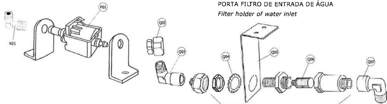
(R01) BLOCO DISTRIBUIDOR Distribution unit
