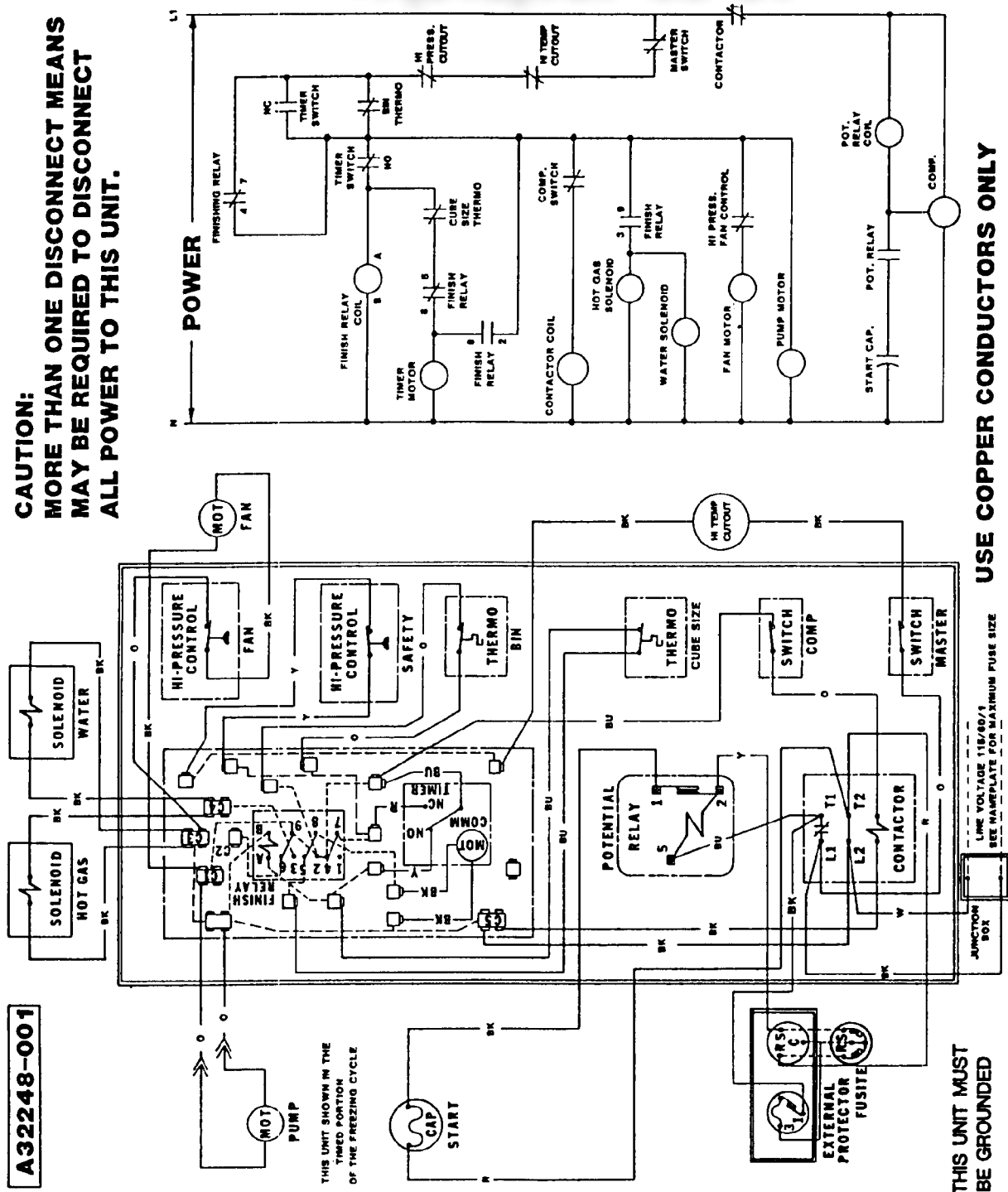
Wiring Diagram CM250AE-1D and CM250AE-1E (115/60/1)
