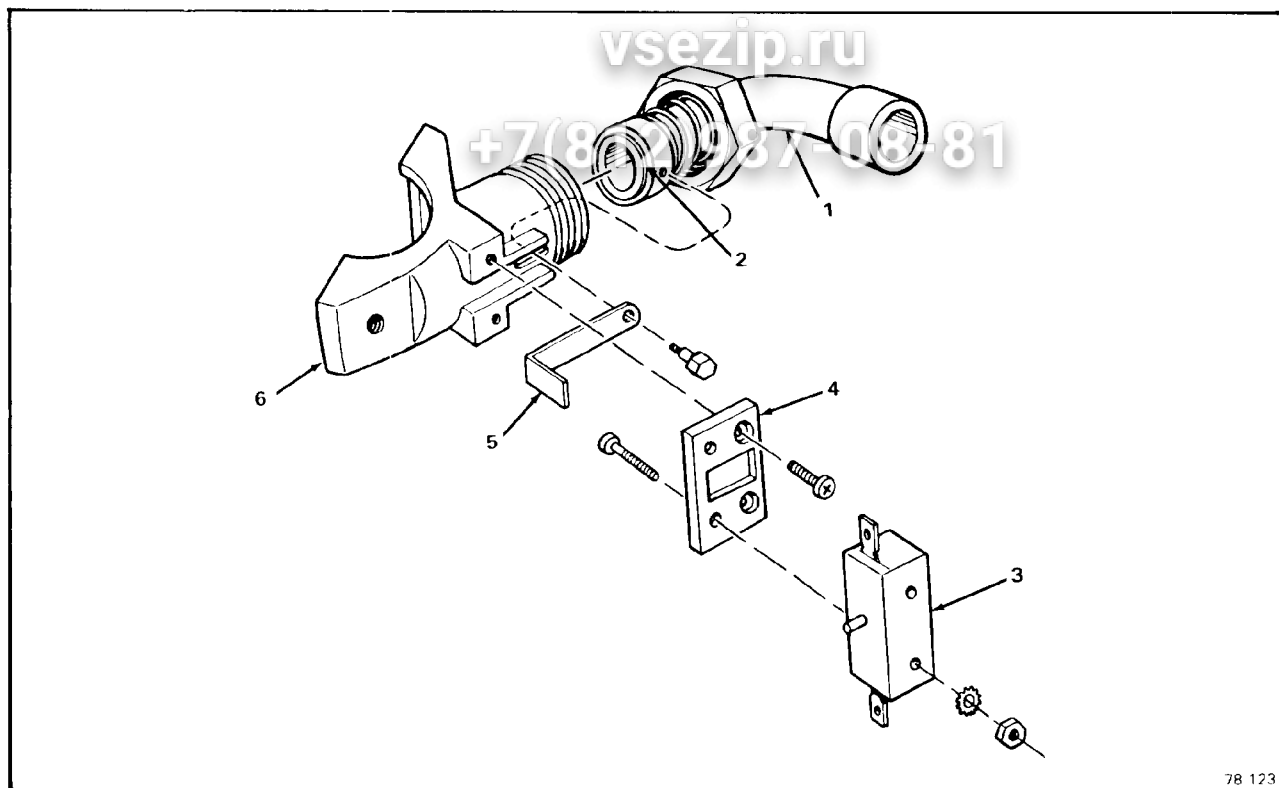
Figure 8-5. Spout Assembly.
