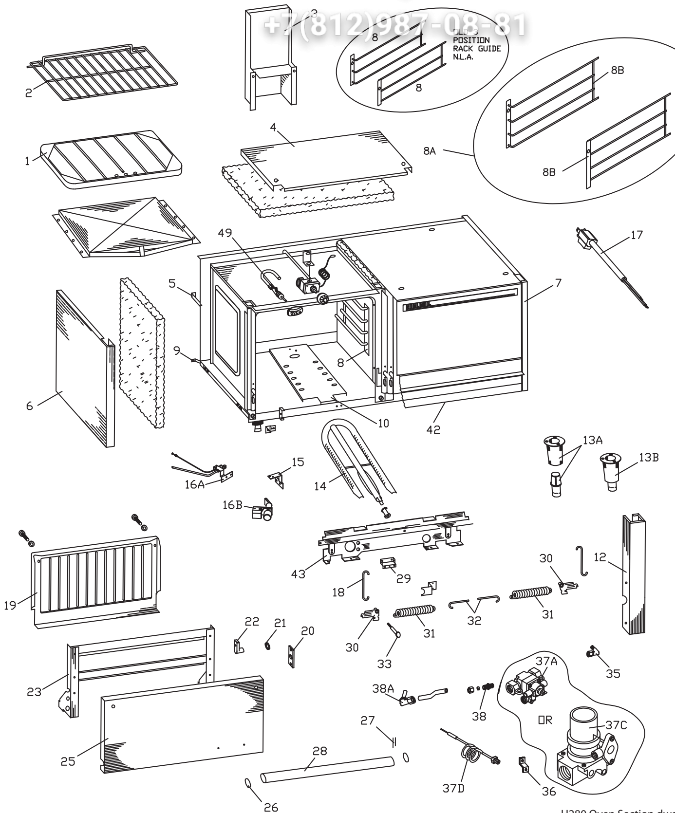
H280 Oven Section.dwg
