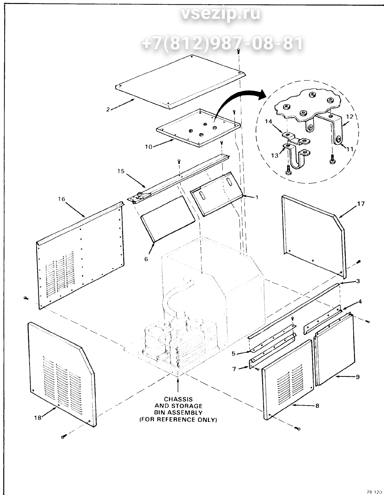
Figure 8-1. AF-430 Cabinet.
